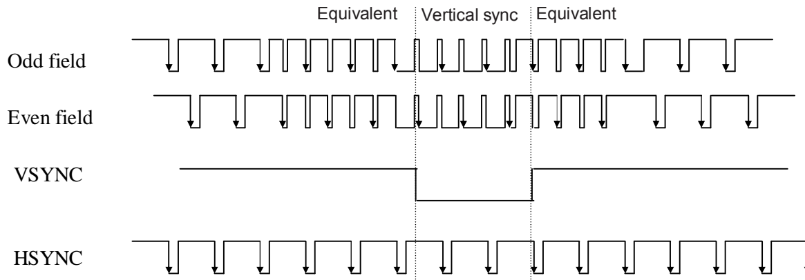
Fig. 6: CSYNC Data input format
