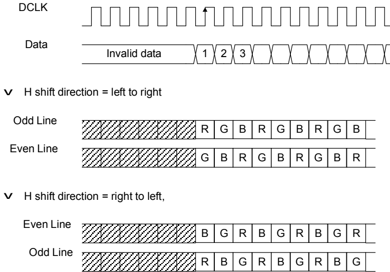
Fig. 10 UPS051 Input RGB sequence for 960x240 resolution
