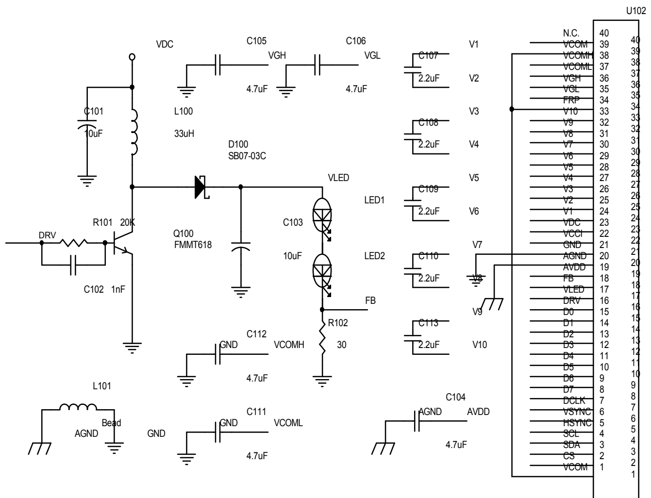
Fig.12 Typical Application Circuit
