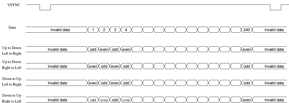
Fig 9. UPS051 even and odd lines definition
