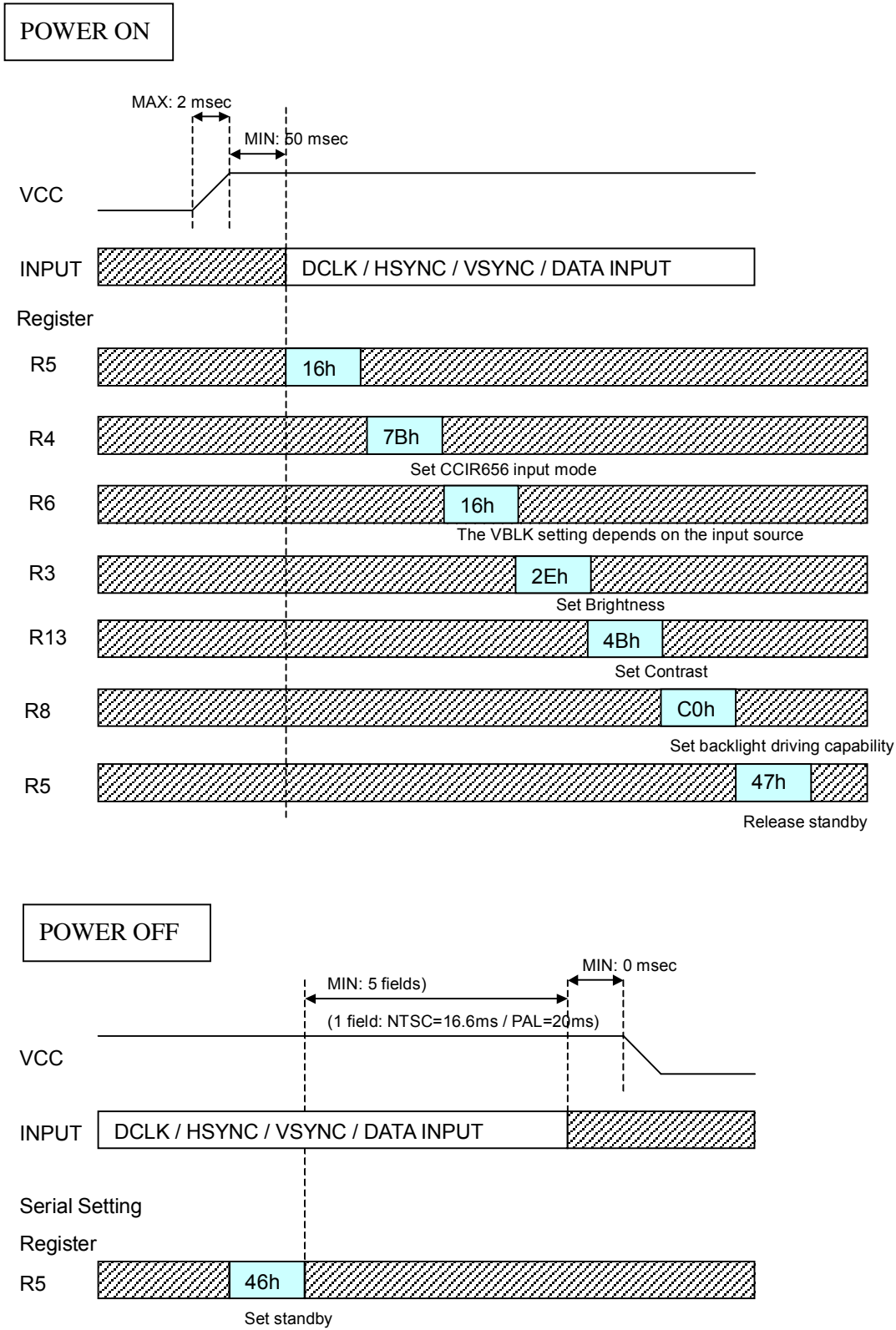
Fig.17 Recommend serial command settings for CCIR656
